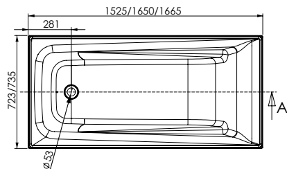
novara - 1525 x 735 x 447mm 1650 x 735 x 447mm & 1650 x 723 x 435mm
