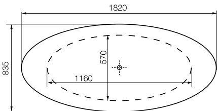
munich - 1820 x 835 x 765mm
