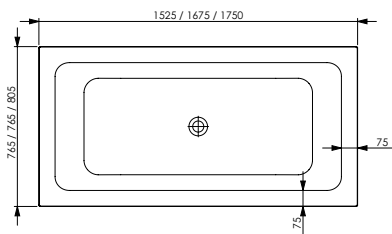
carina - 1525 x 765 x 440mm 1675 x 765 x 440mm & 1750 x 805 x 480mm
