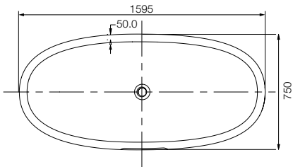
sheraton - 1595 x 750 x 625mm
