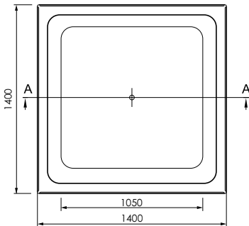
venice - 1400 x 1400 x 520mm
