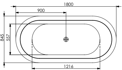
caval - 1800 x 845 x 485mm
