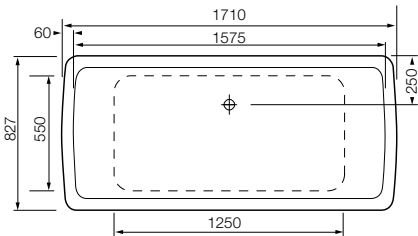
westin - 1710 x 827 x 615mm
