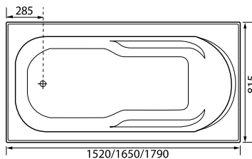
prima - 1520 x 815 x 445mm 1650 x 815 x 510mm & 1790 x 815 x 510mm
