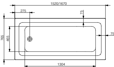
cortez - 1520 x 765 x 450mm 1670 x 765 x 450mm
