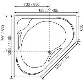
angelique - 1295 x 1295 x 480mm 1465 x 1465 x 480mm
