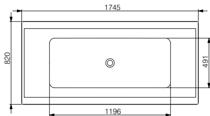
martino - 1745 x 820 x 485mm
