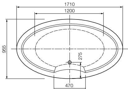
oval - 1710 x 955 x 622mm
