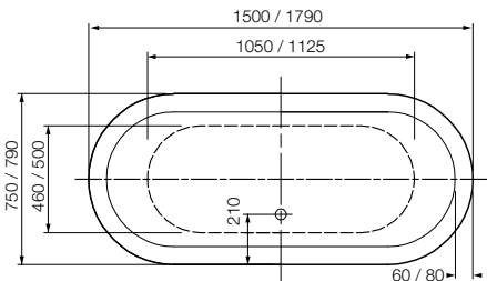
cool - 1500 x 750 x 600mm 1790 x 790 x 590mm
