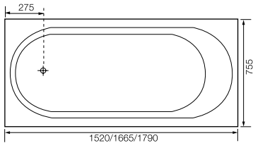
turin - 1520 x 755 x 445mm 1665 x 755 x 445mm & 1790 x 755 x 445mm
