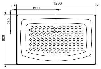
azzurro rectangle - 1200 x 820 x 425mm Not available as a spa.
