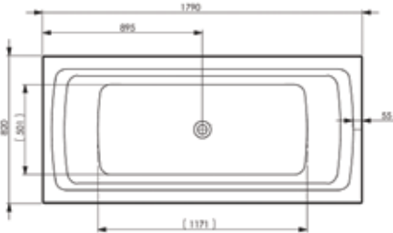
san diego - 1790 x 820 x 495mm
