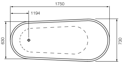
sarto - 1750 x 730 x 750mm
