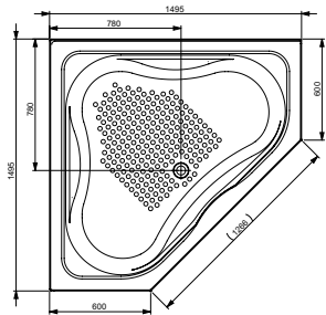
renee - 1495 x 1495 x 495mm
