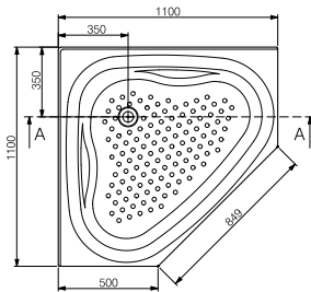
azzurro corner - 1100 x 1100 x 455mm Not available as a spa.
